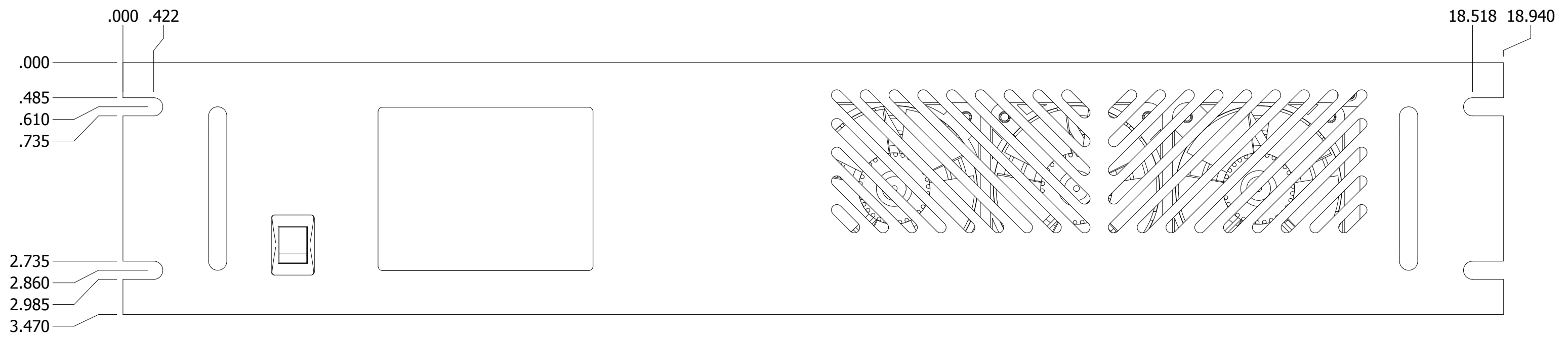
FRONT SCALE 0.75:1
